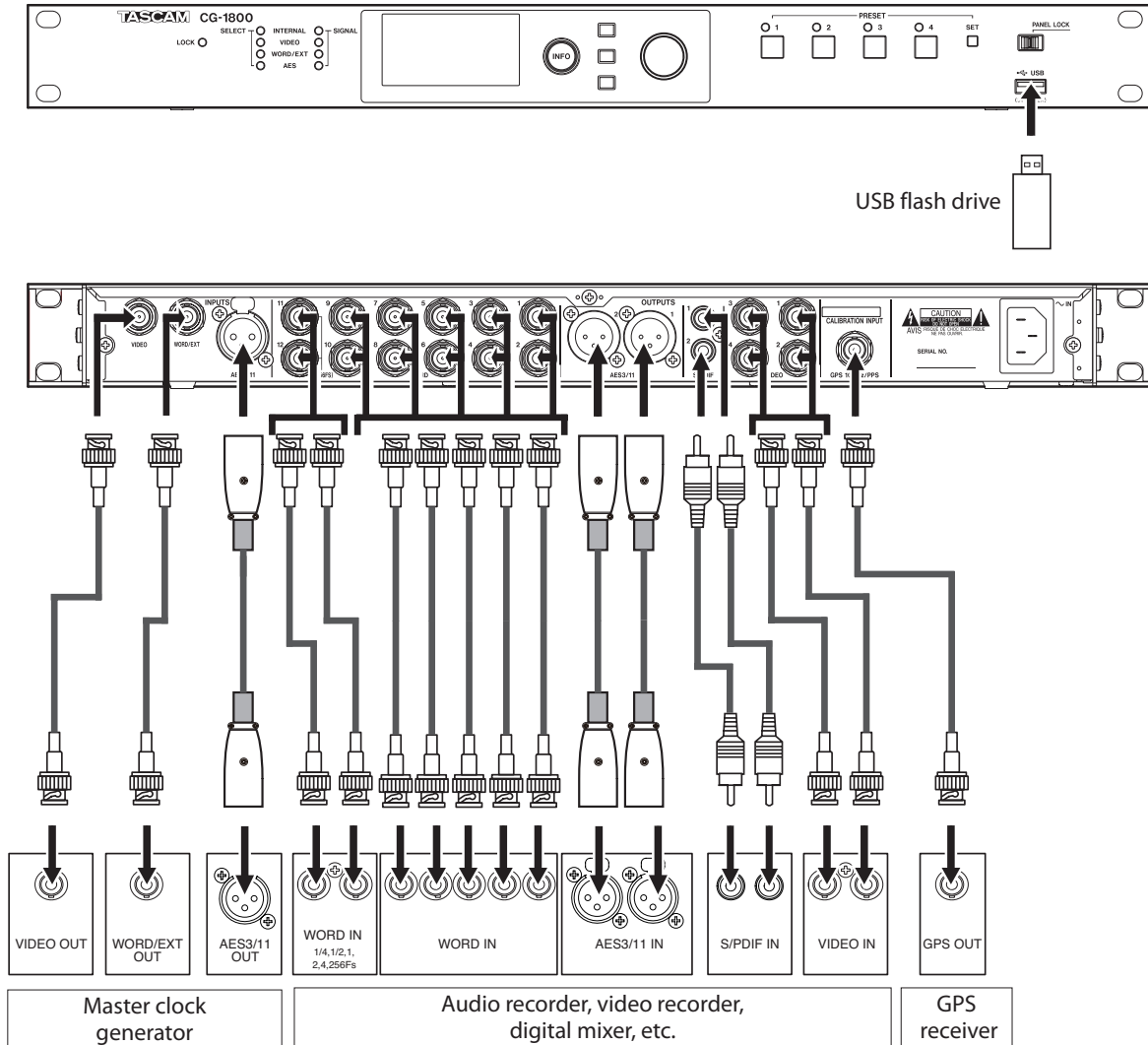
CG-1800 connection example
